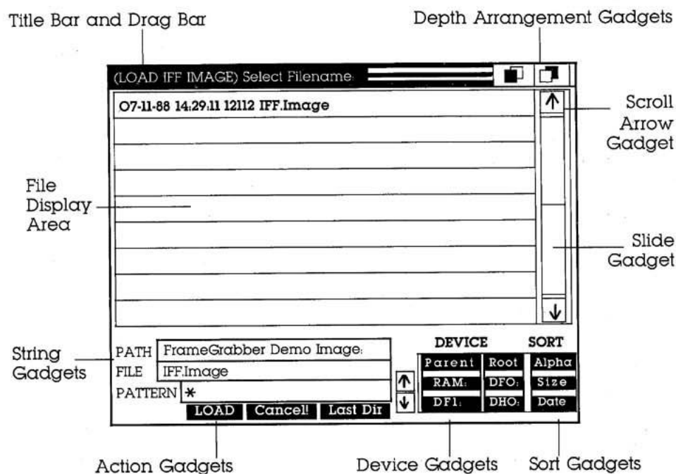
Figure 4 Path-Master File Selector
